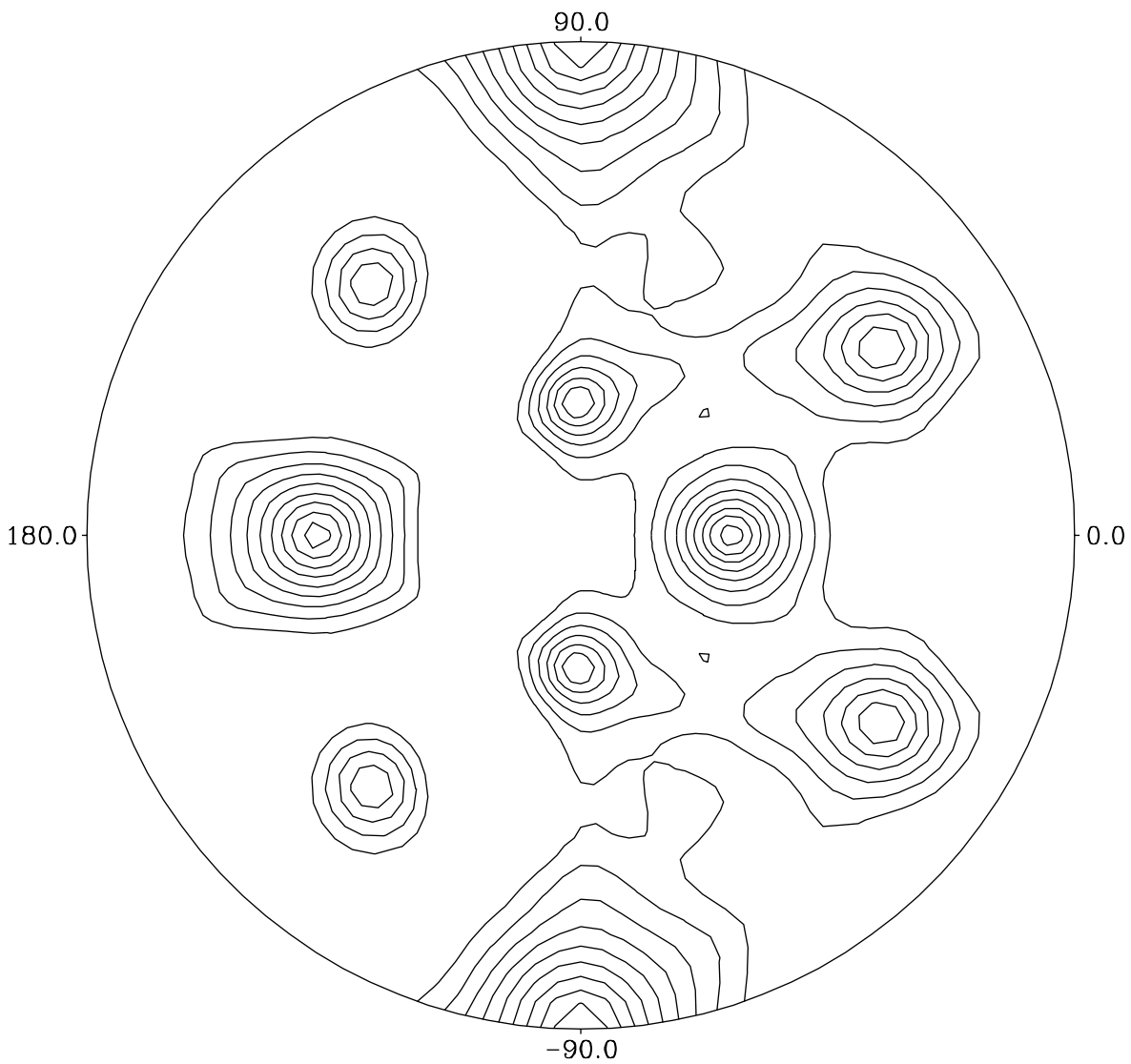
Self_rotation function on EhaAc native xtal23 Section kappa = 180
