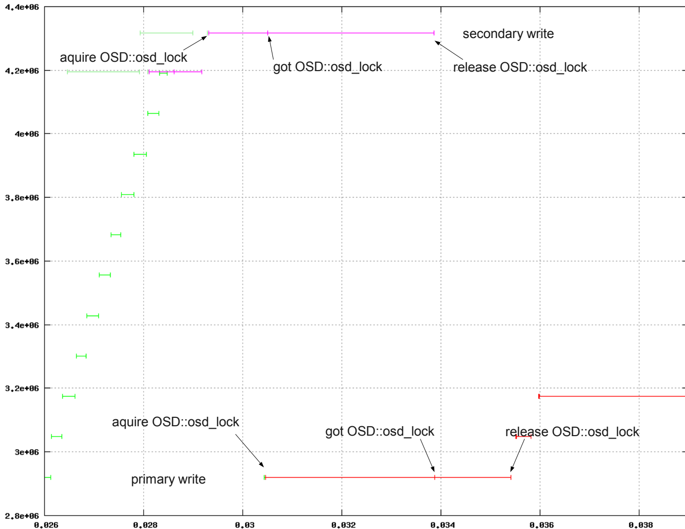
osd.0: primary writes of sequential io-test ; client CFQ
