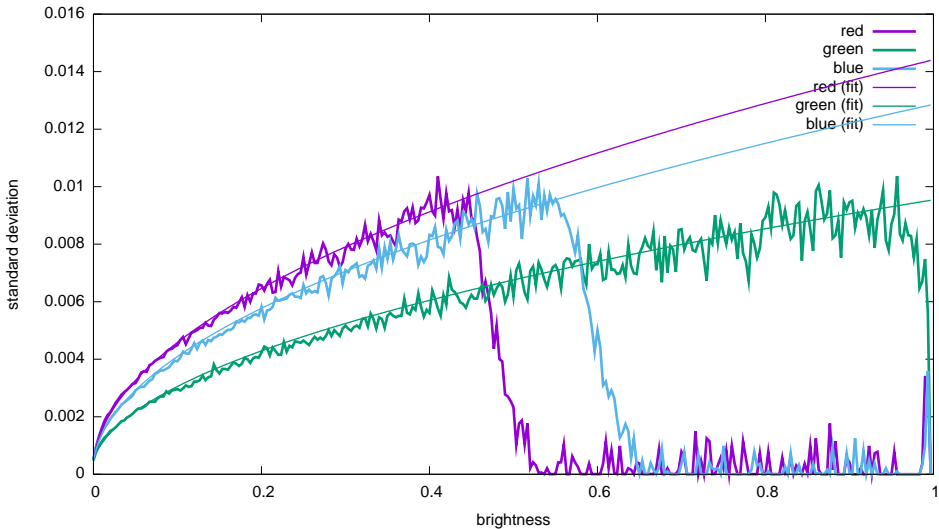
Noise levels - Apple, iPhone 6s, 2000 ISO (07012017164604)
