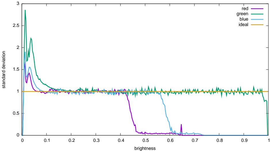
Flat noise levels - Apple, iPhone 6s, 200 ISO (07012017164149)
