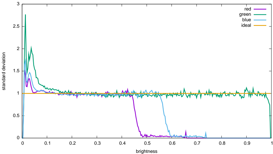
Flat noise levels - Apple, iPhone 6s, 2000 ISO (07012017164604)
