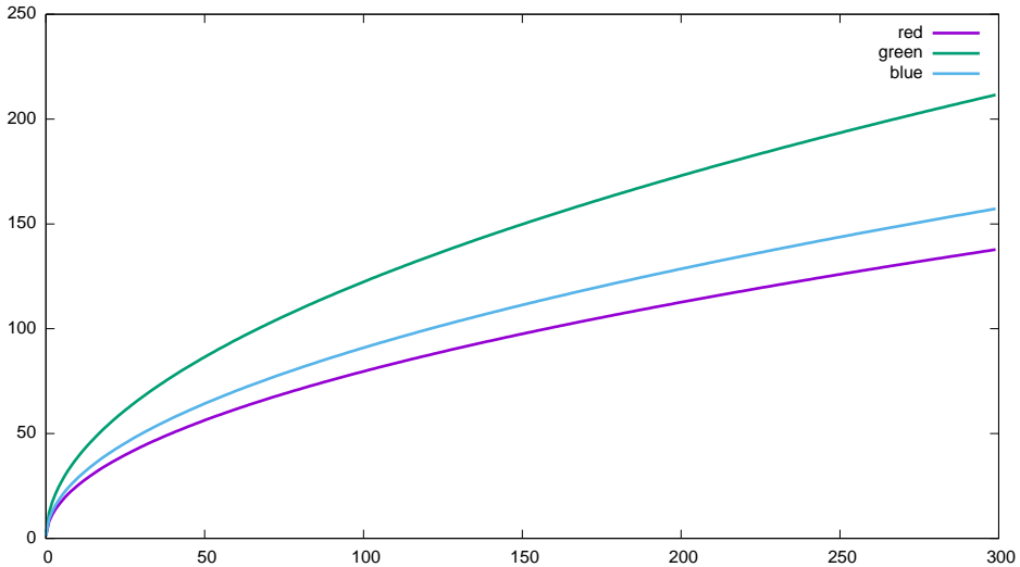
Conversion curves - Apple, iPhone 6s, 200 ISO (07012017164149)
