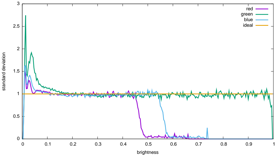
Flat noise levels - Apple, iPhone 6s, 1600 ISO (07012017164150)
