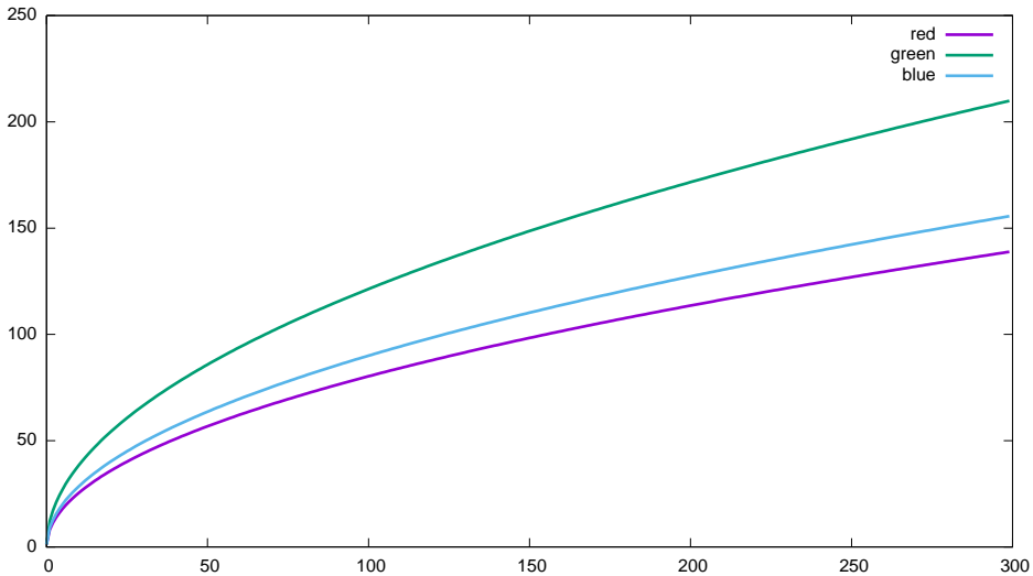
Conversion curves - Apple, iPhone 6s, 2000 ISO (07012017164604)
