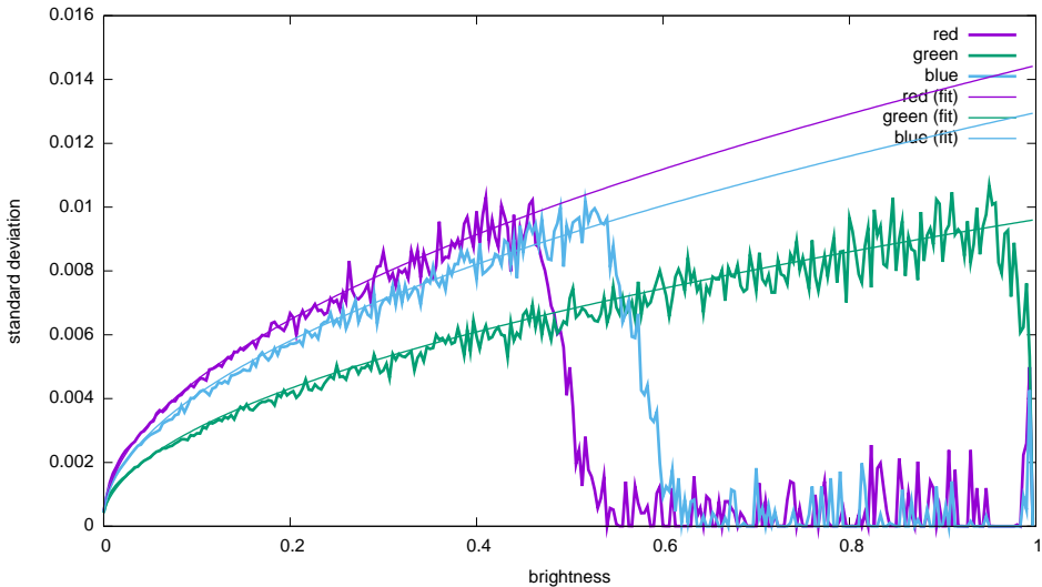
Noise levels - Apple, iPhone 6s, 1600 ISO (07012017164150)
