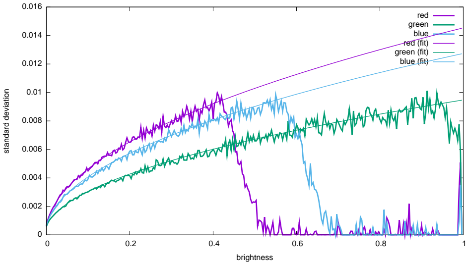
Noise levels - Apple, iPhone 6s, 200 ISO (07012017164149)
