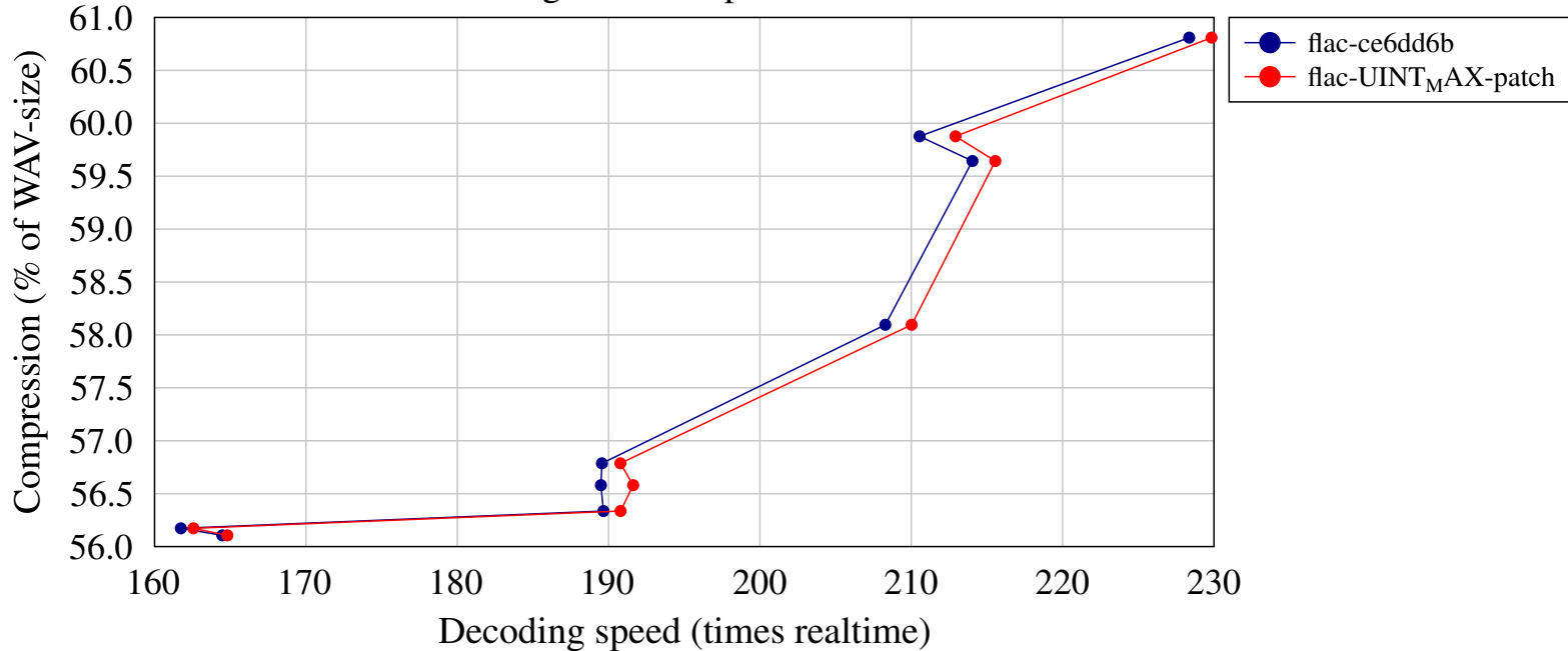
Decoding speed vs compression for long set of samples 2
