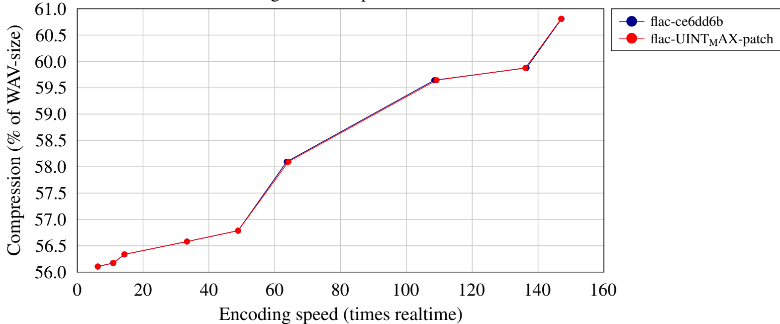
Encoding speed vs compression for long set of samples 2
