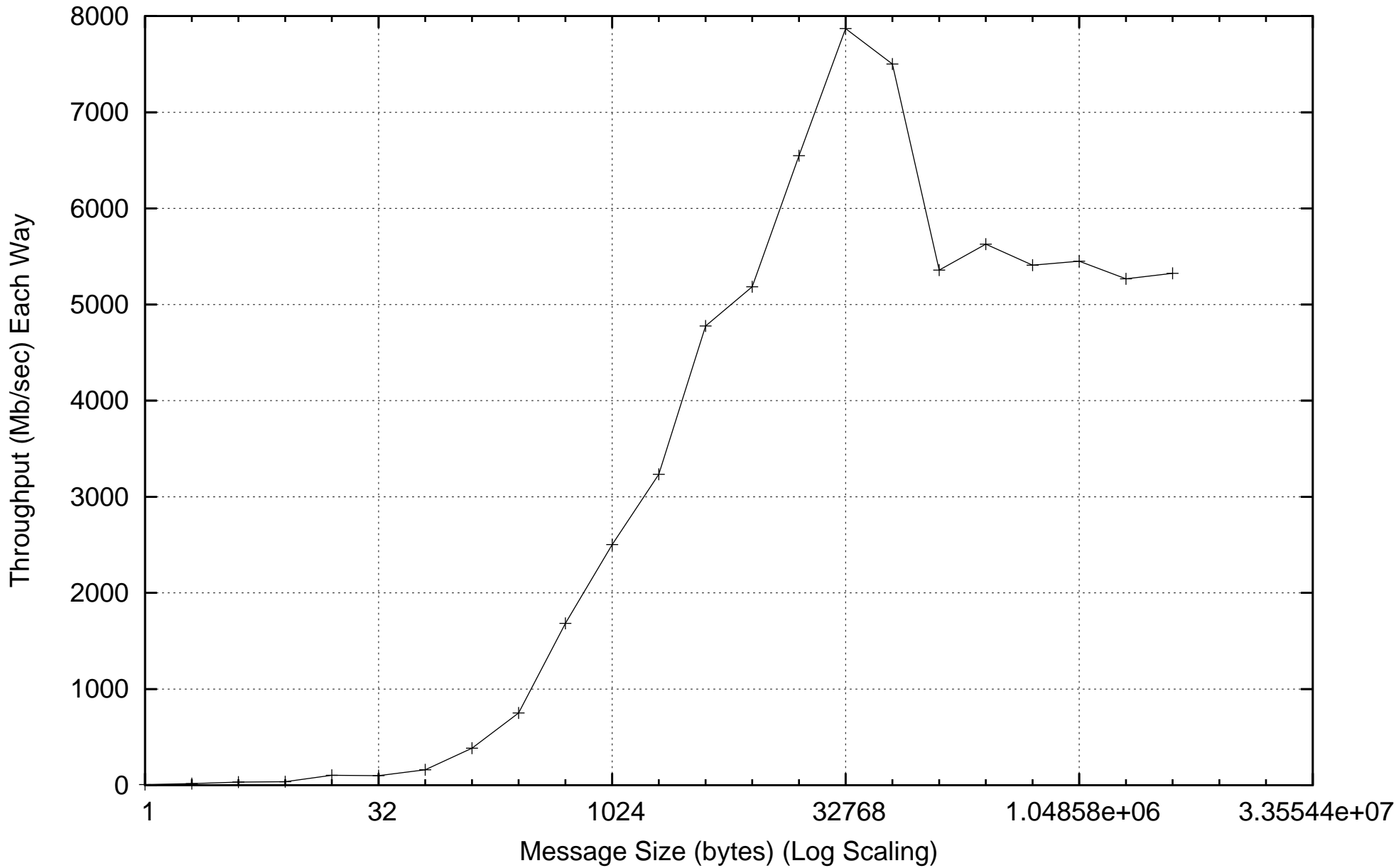
sdp2sdp netperf TCP_STREAM Benchmarks From svbu-qa1950-2 to svbu-qa1950-1, OFED-1.2 buildalpha1
