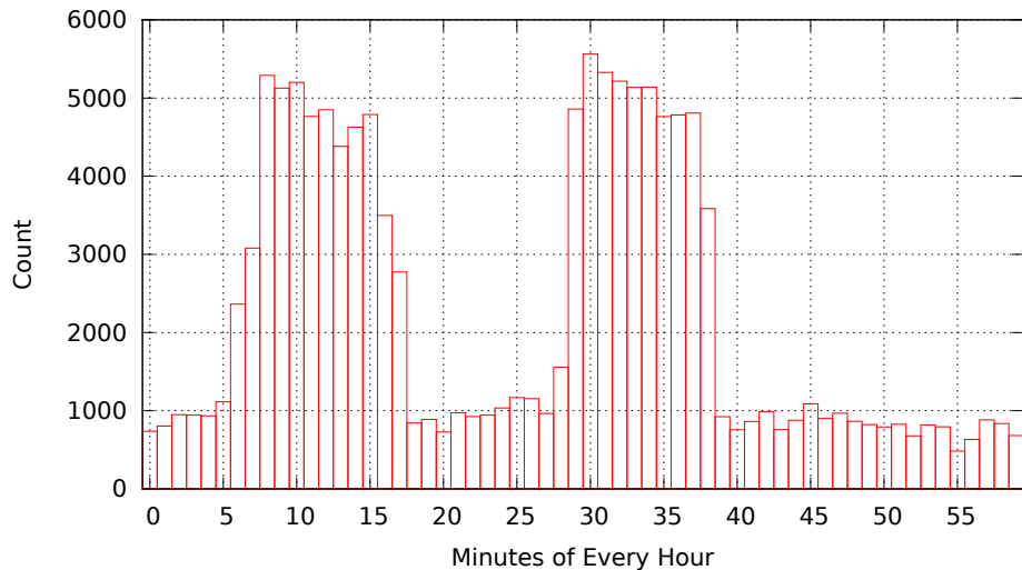
Lookup Failures
