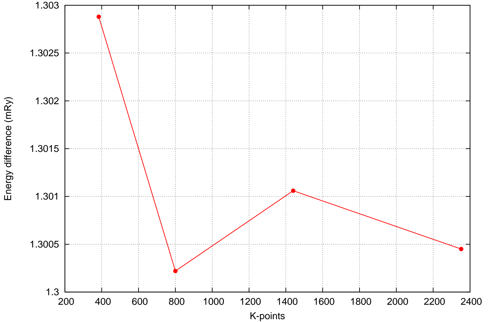
K-point sampling convergent test
