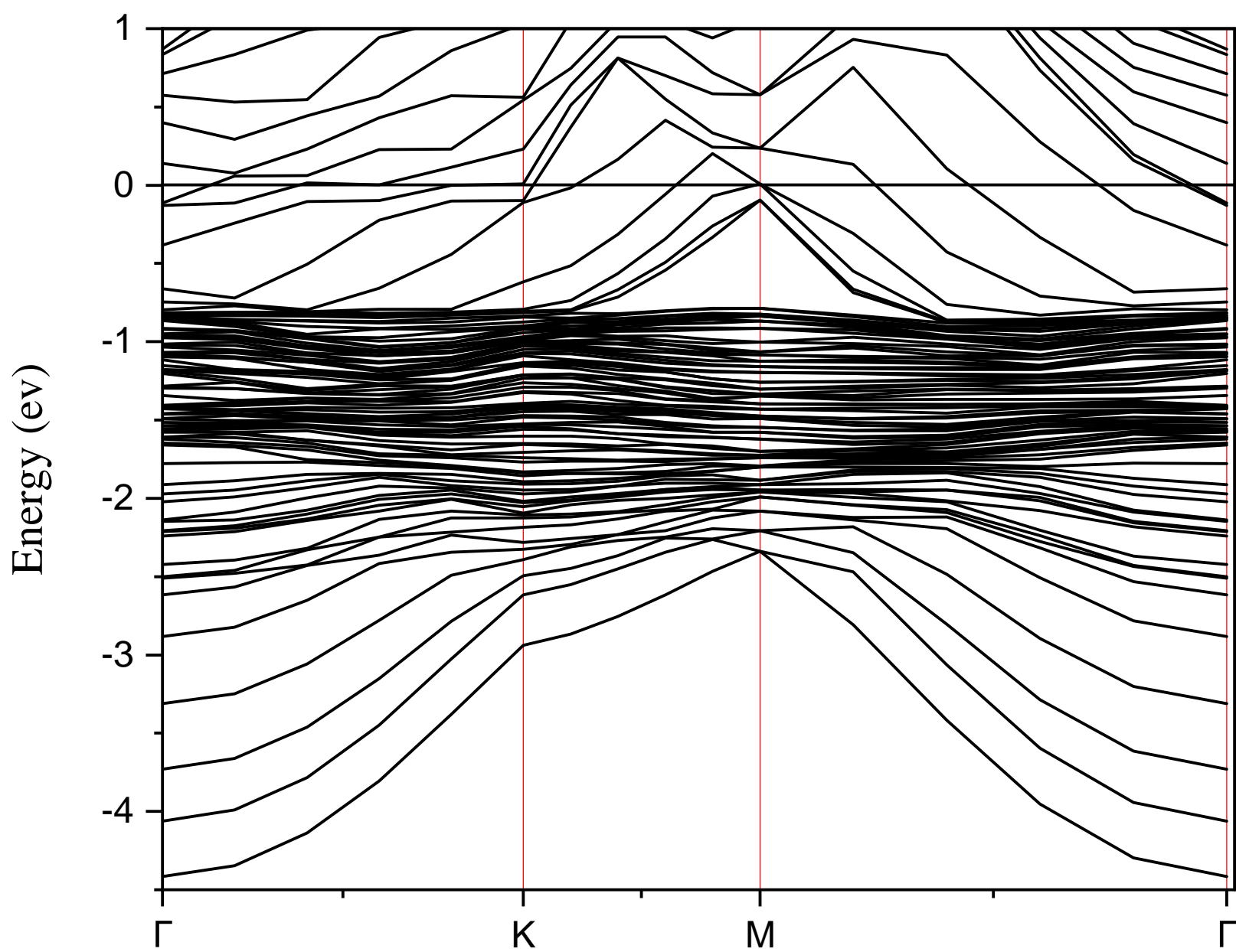
Band structure of Cu(111) with 7 layers
