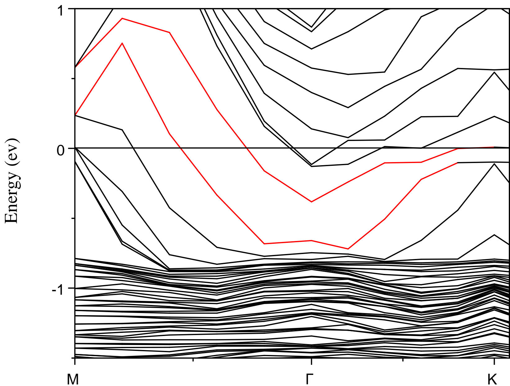
Band structure of Cu(111) with 7 layers
