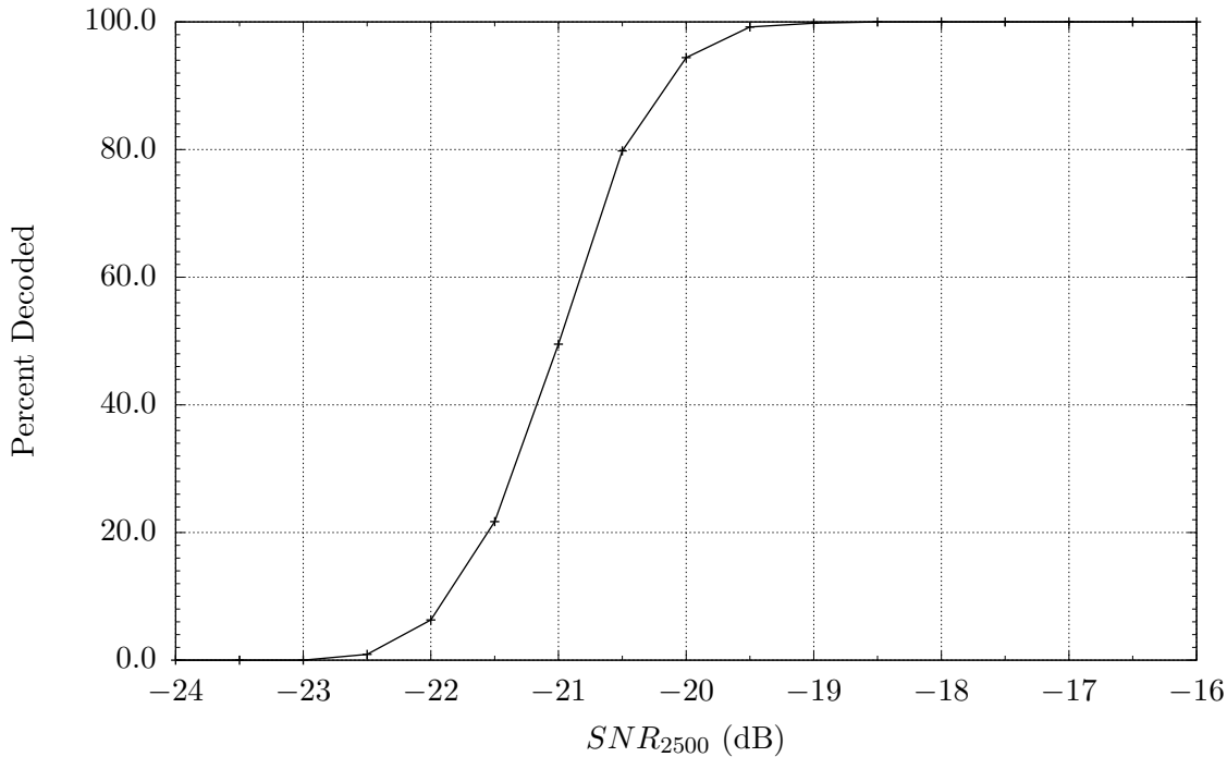
FT8 AWGN decoding - r7775
